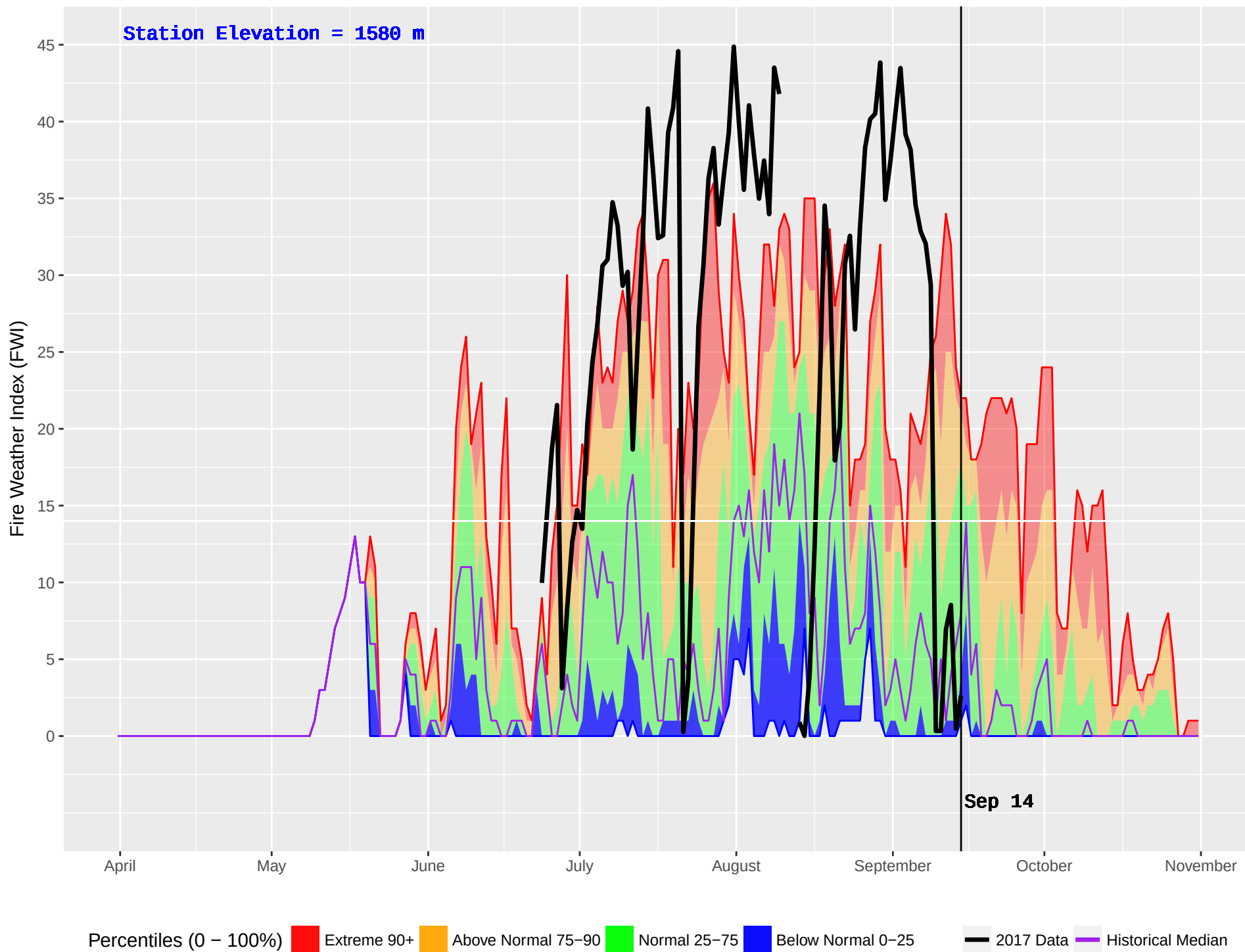
RORY CREEK (1092) : Historical (2010–2016) and Current (2017) Noon Fire Weather Index (FWI)
